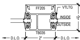
VERTICAL 4-1
