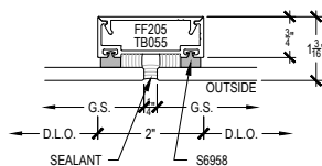
SSG VERTICAL 4-2
