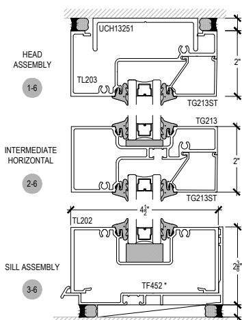
SCREW SPLINE INSIDE SET
