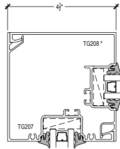
90° CORNER SCREW RACE ASSEMBLY
