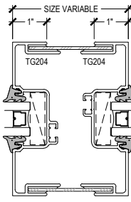
VARIABLE VERTICAL ASSEMBLY
