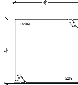
4 1/2" TUBE ASSEMBLY
