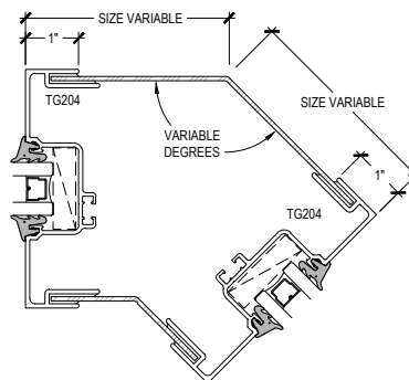
FLEXIBLE CORNER ASSEMBLY
