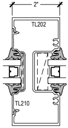
INTERMEDIATE VERTICAL
