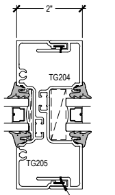
EXPANSION VERTICAL ASSEMBLY
