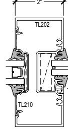
INTERMEDIATE VERTICAL w/ADAPTOR AND GLASS OPTION
