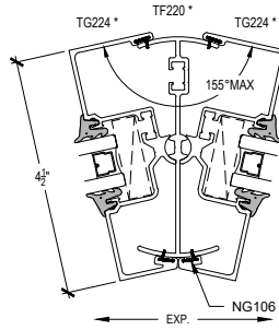
180-155° FLEXIBLE CORNER ASSEMBLY
