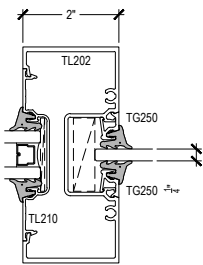
INTERMEDIATE VERTICAL w/ADAPTOR AND GLASS OPTION
