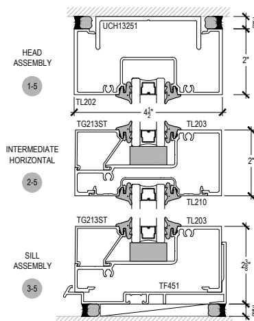
SCREW SPLINE OUTSIDE SET
