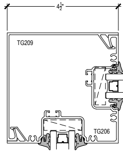
90° CORNER ASSEMBLY
