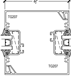
4 1/2" VERTICAL ASSEMBLY
