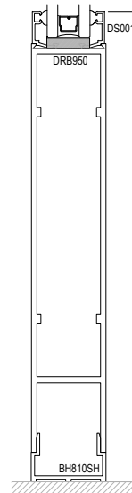
SIDELIGHT BOTTOM RAIL
