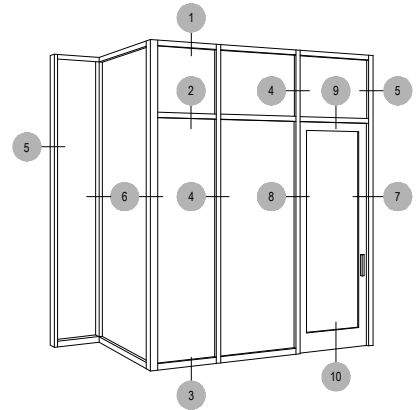
INTERMEDIATE VERTICAL w/ADAPTOR AND GLASS OPTION
