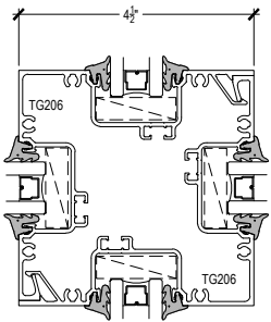
SPECIAL ASSEMBLY
