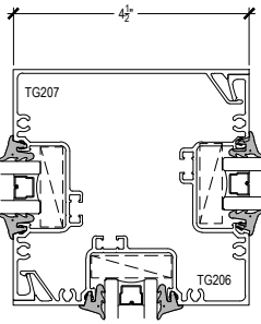
SPECIAL ASSEMBLY
