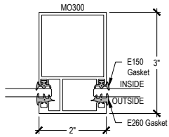
INTERMEDIATE VERTICAL
